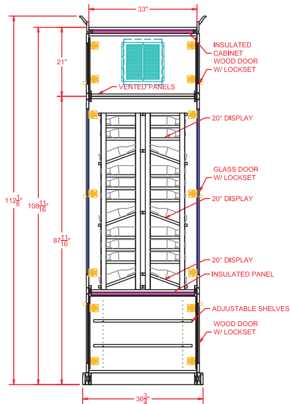
SECTION -1-
