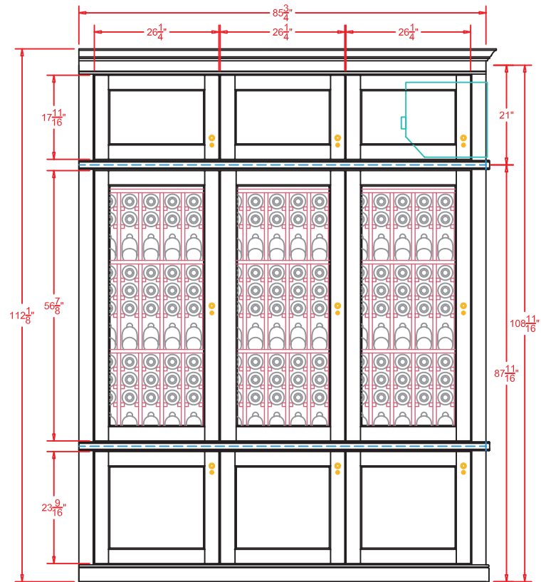
ELEVATION (OPPOSITE SIDE IS MIRROR)
